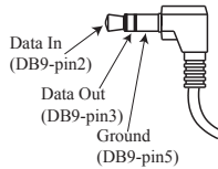
Figure 08– Mini plug for RS232 connection
