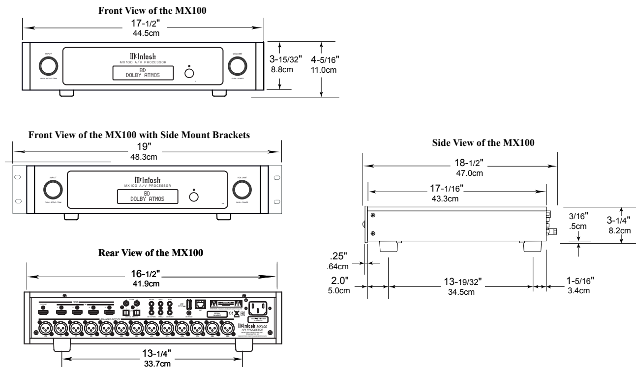
Figure 01– MX100 Dimensions
