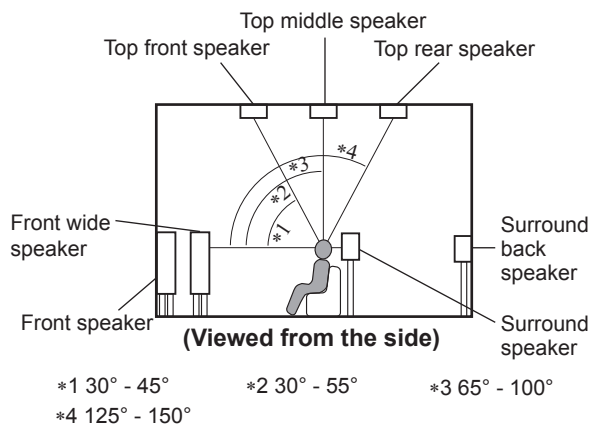
Figure 20– Speaker angles
