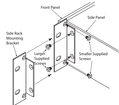
Figure 04– Installing Rack Mount Bracket
