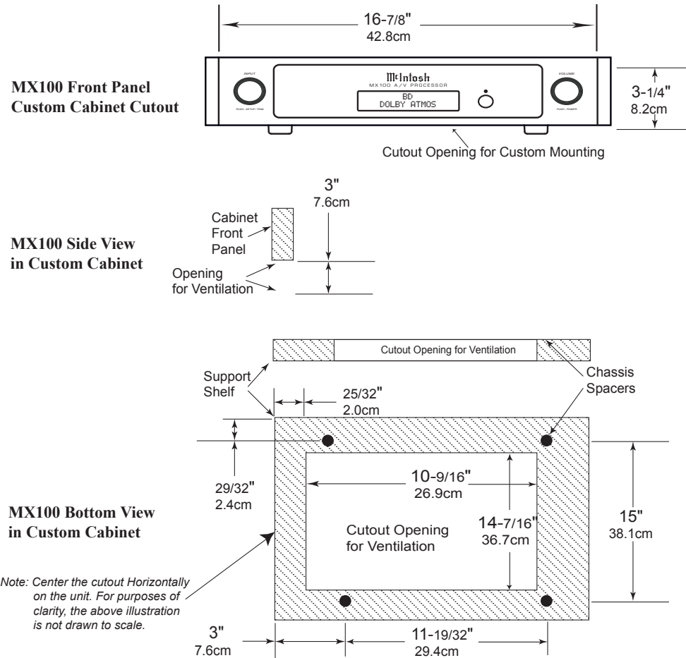
Figure 02– Custom cutout dimensions
