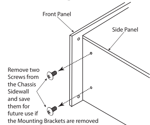
Figure 03– Rack Mount screws
