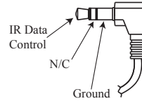
Figure 10– IR 3.5mm connector
