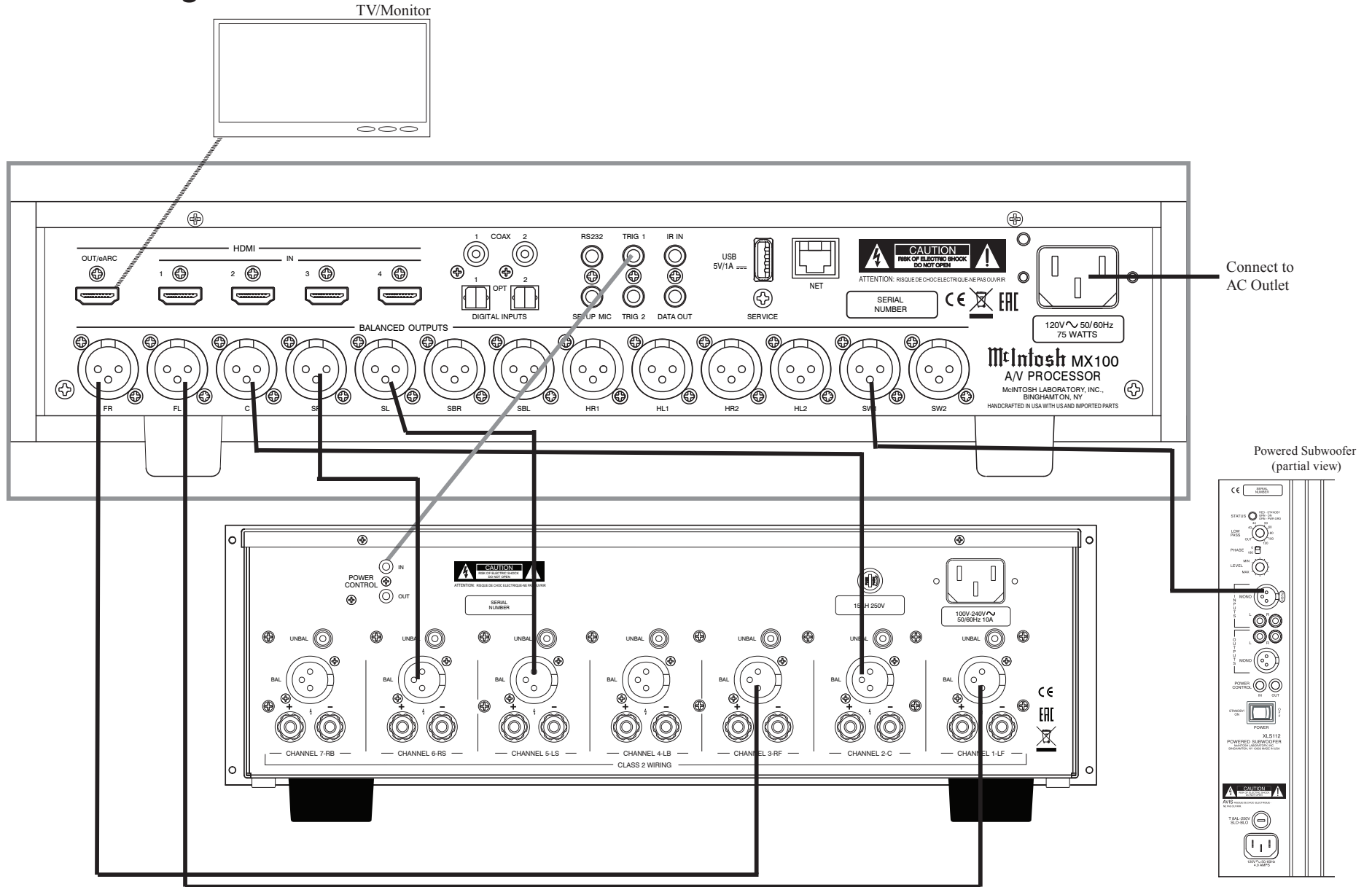
Figure 07– Example 5.1 connection diagram
